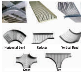
Cable Tray Accessories
